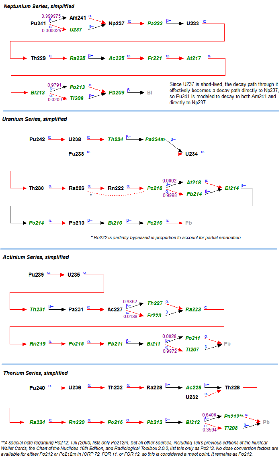
Figure 9: Principal decay chains for the four actinide series. Radionuclides in black are included in the fate and transport model, and those in green are considered only in the dose model.
